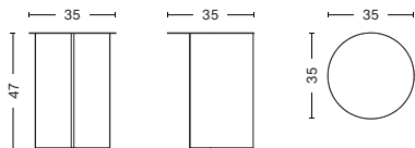
SLIT TABLE ROUND HIGH DIAMETER 35 CM | 13.78" HEIGHT 47 CM | 18.50"
