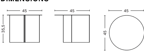
SLIT TABLE ROUND DIAMETER 45 CM | 17.72" HEIGHT 35,5 CM | 13.98"
